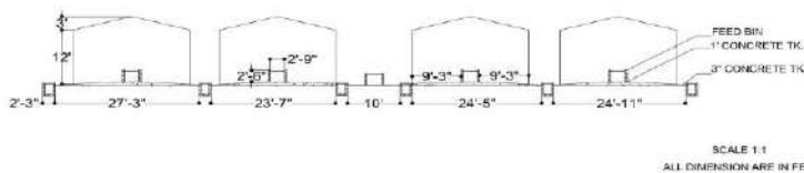
C/S OF SEWAGE AND FEED BIN
